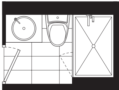
alternate bath option 205 - 705 & 206 - 706
